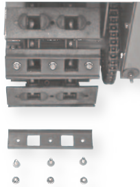
Grouser Shoe TS058
